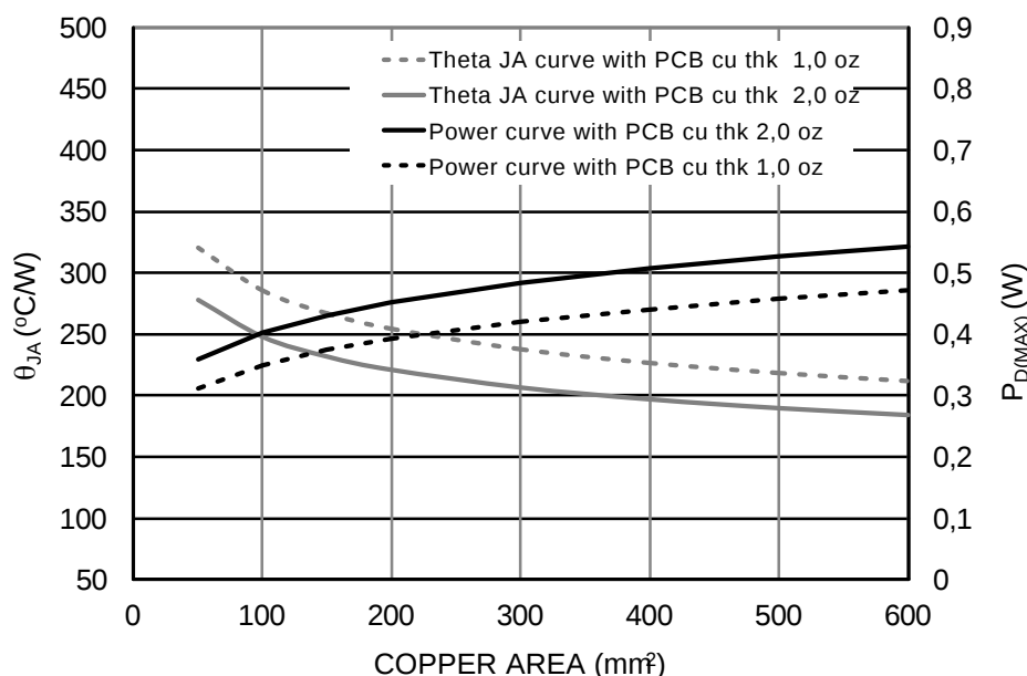
Figure 54. Thermal Parameters vs. Copper Area
