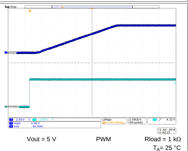
Figure 61. Start-Up Timing
