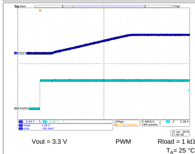
Figure 54. Start-Up Timing
