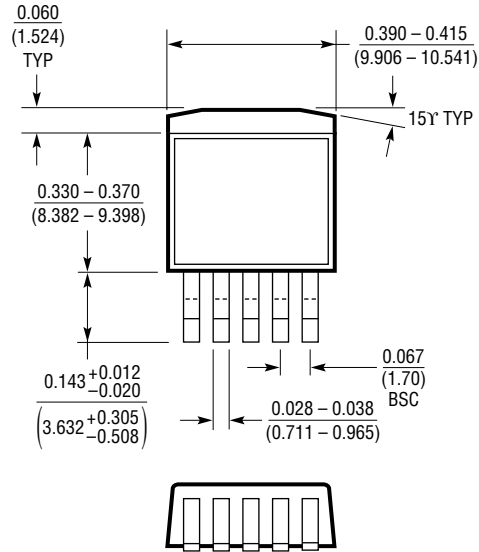
Q Package 5-Lead Plastic DD Pak (Reference LTC DWG # 05-08-1461)
