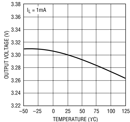
LT1963A-3.3 Output Voltage
